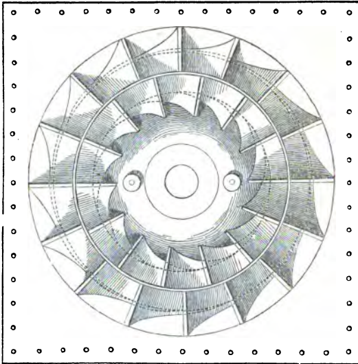
PLAN OF FIXED PART WITH GUIDE CURVES.
